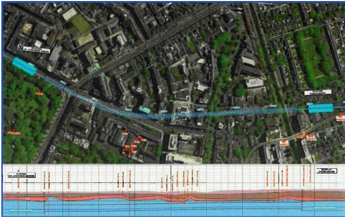
Figure 7. Geological Section (ref. A5.13, Diagram 3.13: Geologic Profile for TBM Drive C8- Tara Station to St Stephen's Green)
